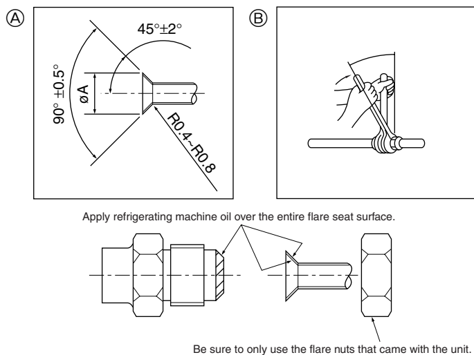
(A) Flare cutting dimensions
