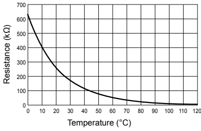
Discharge temperature thermistor (RT62)
