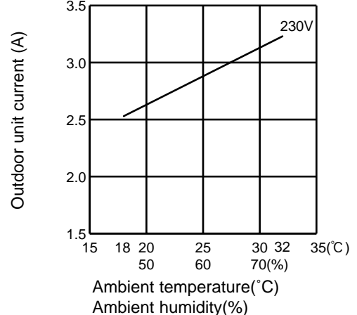
MUH-C09TV -[E1]
