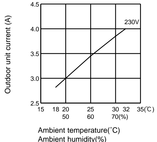
MUH-C09TV -[E1]
