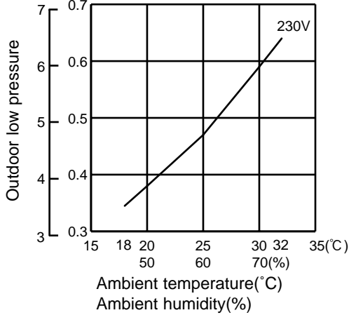
MUH-C07TV -[E1]
