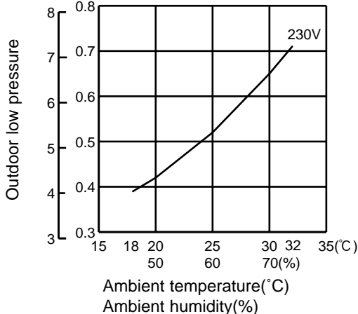
MUH-C09TV -[E1]
