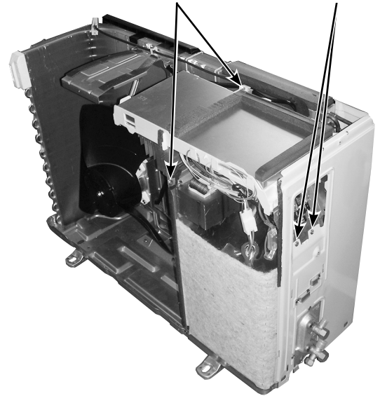
Photo 4 (Inverter assembly)
