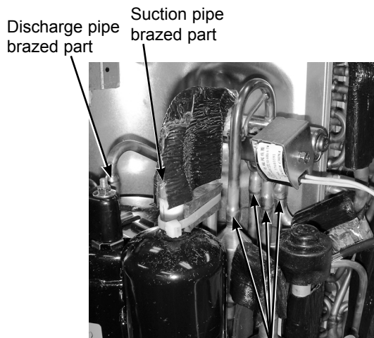
Brazed parts of 4-way valve
