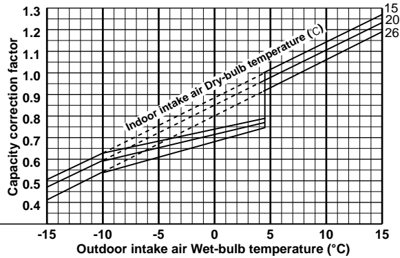
Heating capacity (at Rated frequency)
