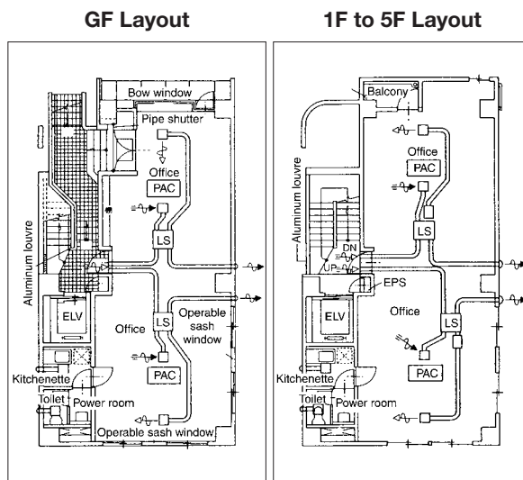
PAC : Package air conditioner LS : Lossnay
