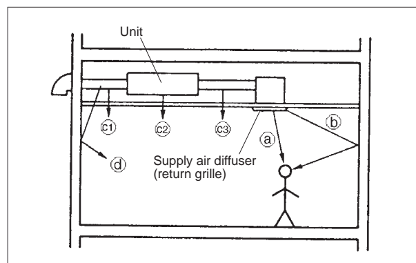
Fig. 3. (Position of Sound Source and Directivity Factor Q)
