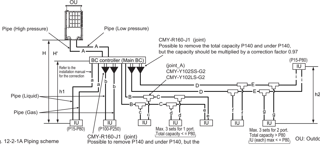
Fig. 12-2-1A Piping scheme
