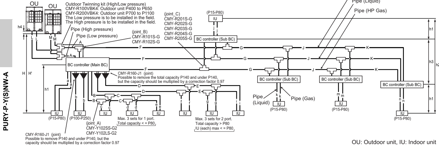
Fig. 12-2-3A Piping scheme
