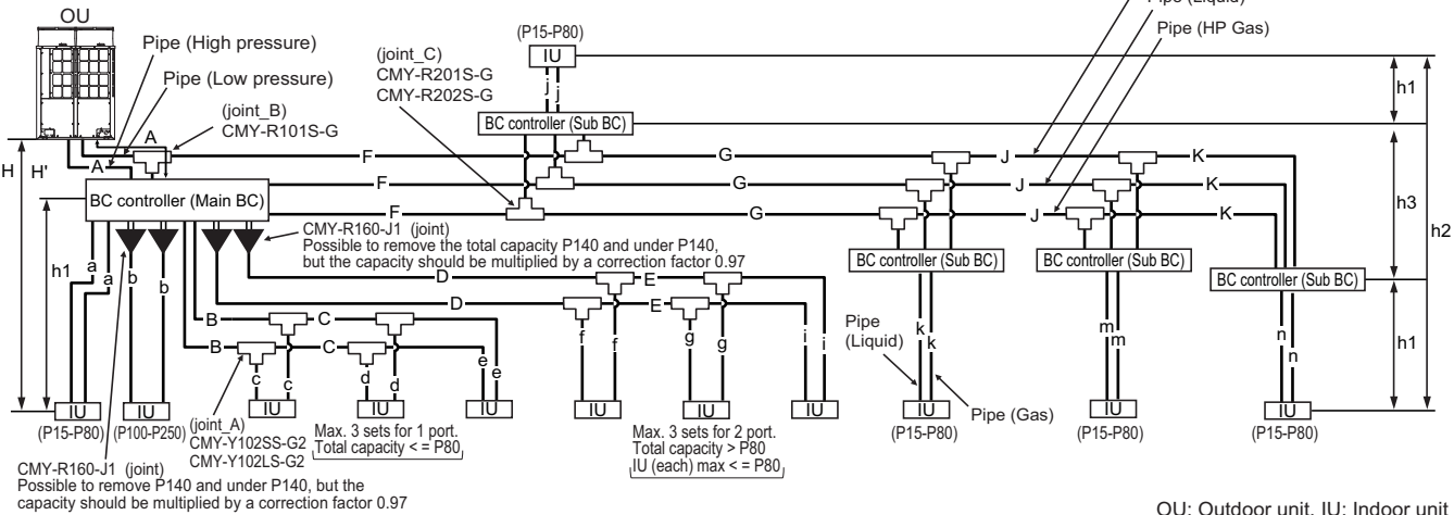
Fig. 12-2-2A Piping scheme
