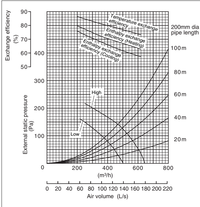
GUF-50RDH3
