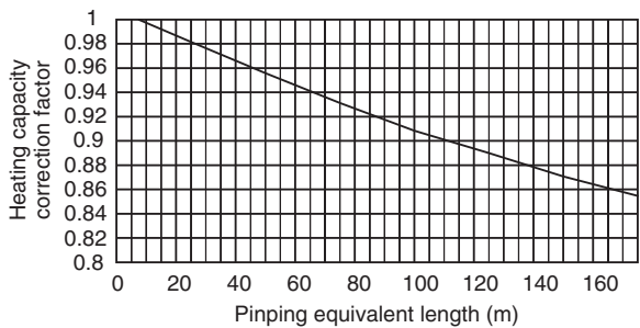
PURY-P450YGM-A, PURY-P500YGM-A
