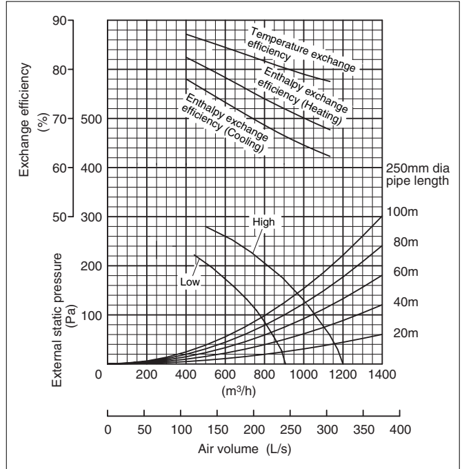
GUF-100RDH3
