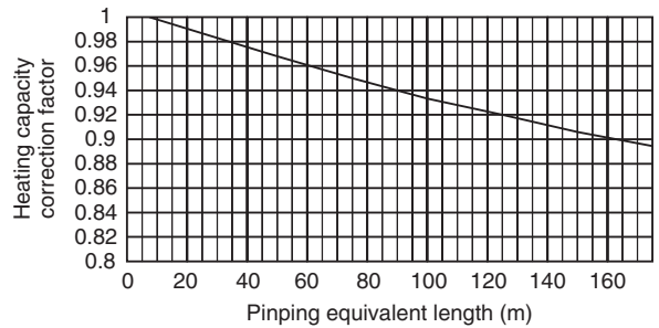
PURY-P350YGM-A, PURY-P400YGM-A
