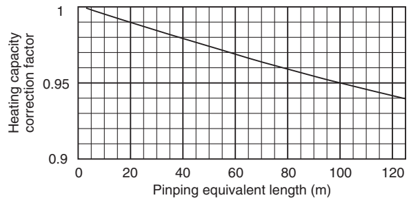
PURY-P350YGM-A, PURY-P400YGM-A
