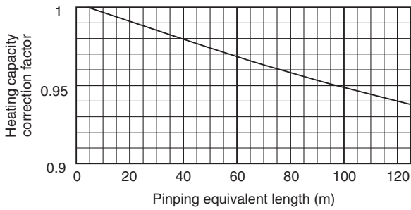
PUHY-P200YGM-A, PUHY-P250YGM-A
